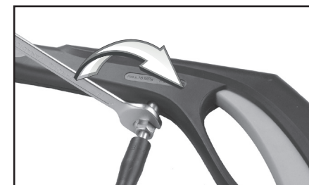
Installation of the pressure hose on model HPC 1800 Fig.8
